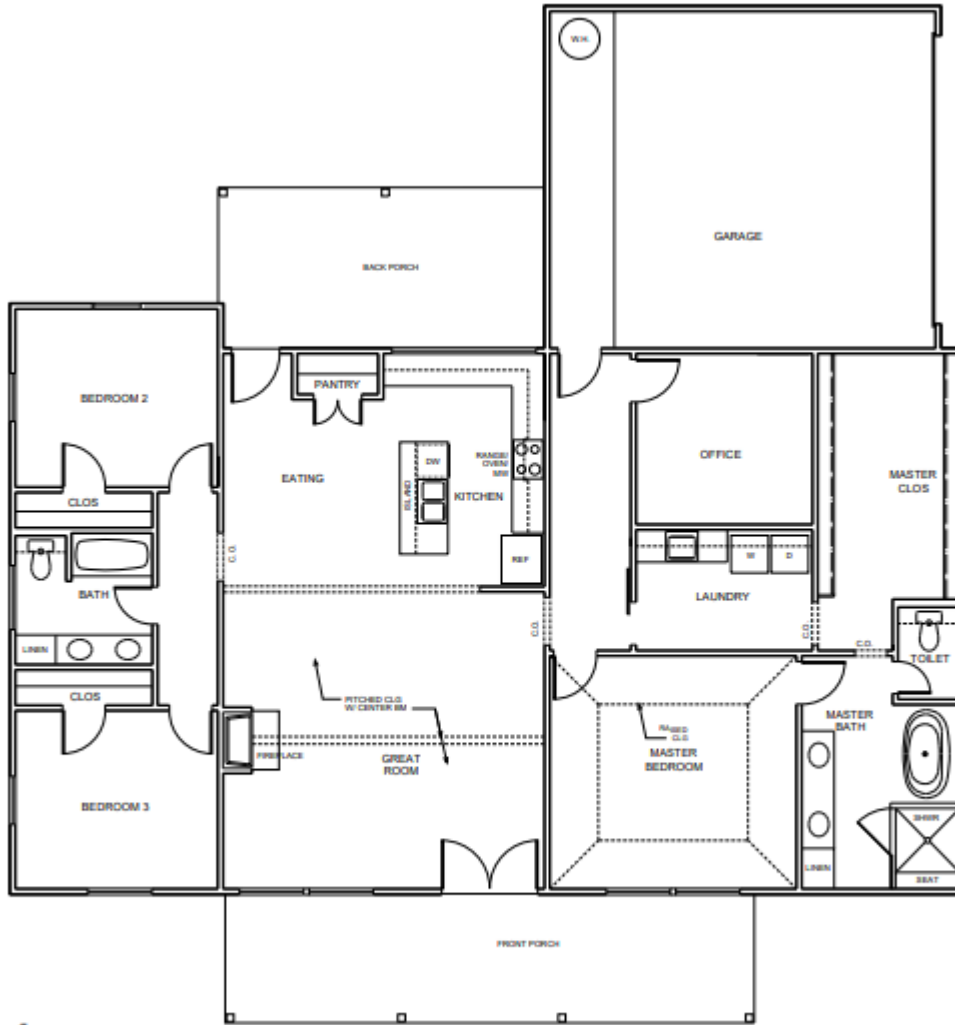
1 FLOOR PLAN 1/4" = 1'-0"
